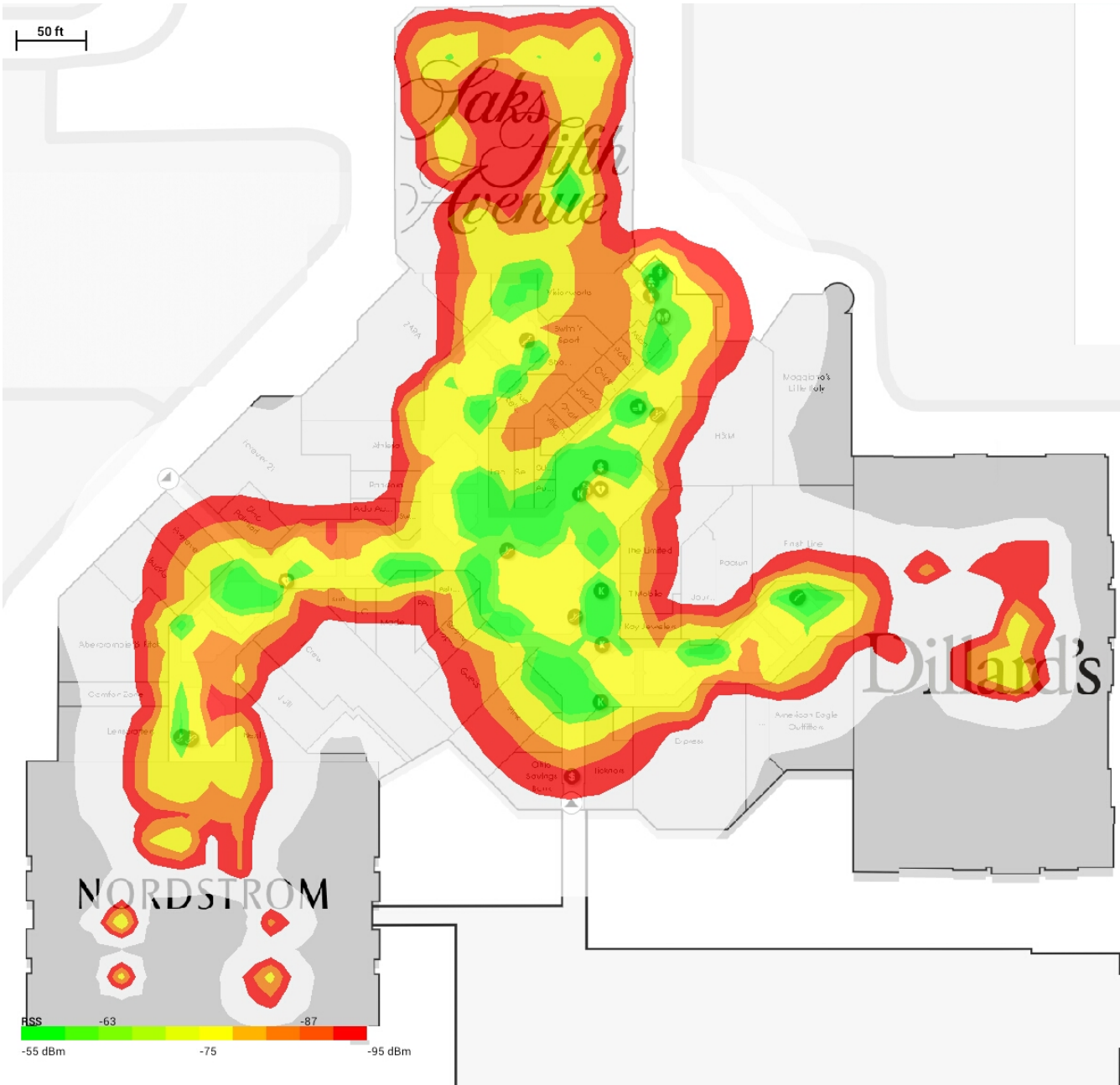
The following snapshot shows the SNR heatmap of Beachwood_L2
